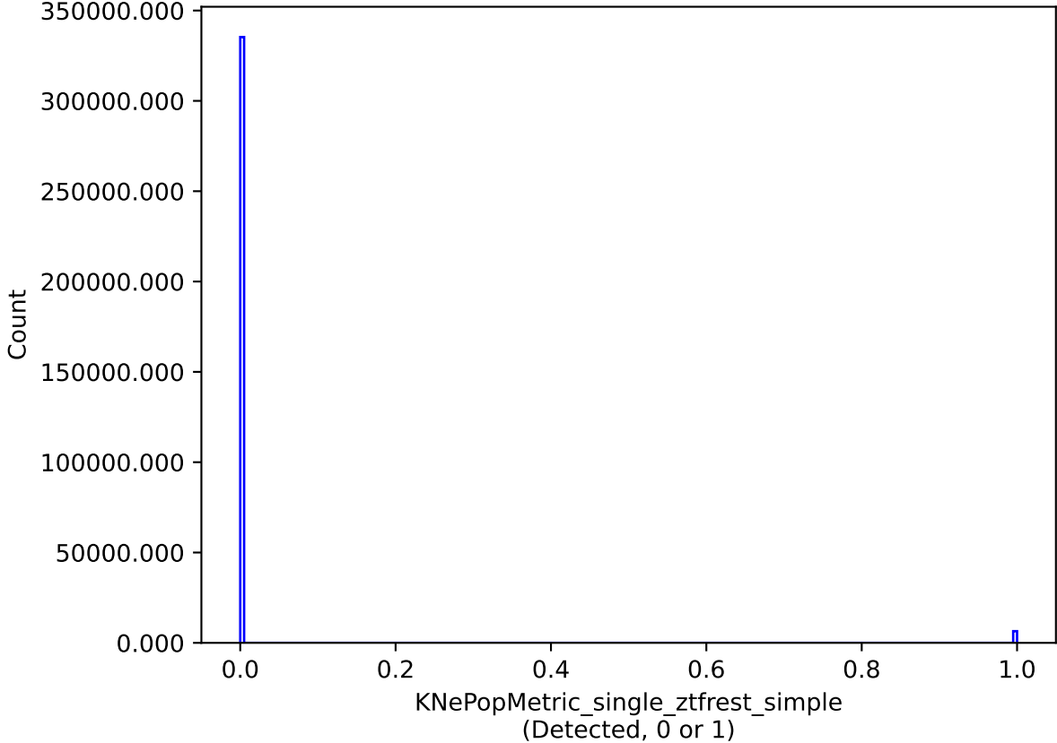
all_long_v3.4_10yrs single model: KNePopMetric_single_ztfrest_simple
