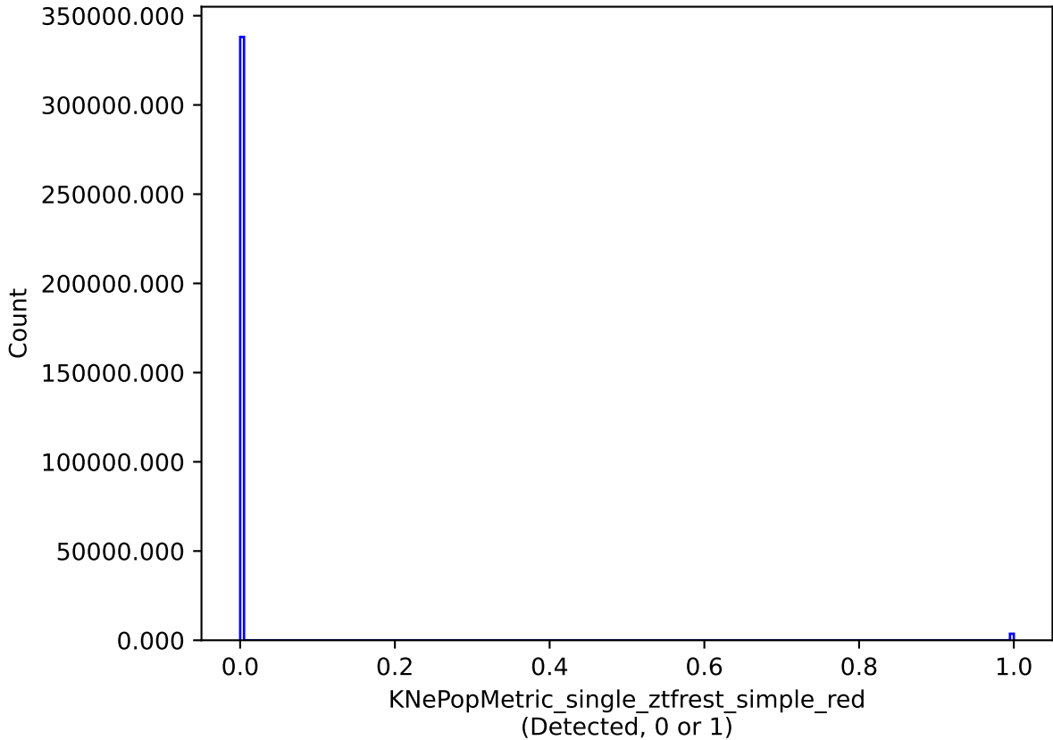
all_long_v3.4_10yrs single model: KNePopMetric_single_ztfrest_simple_red
