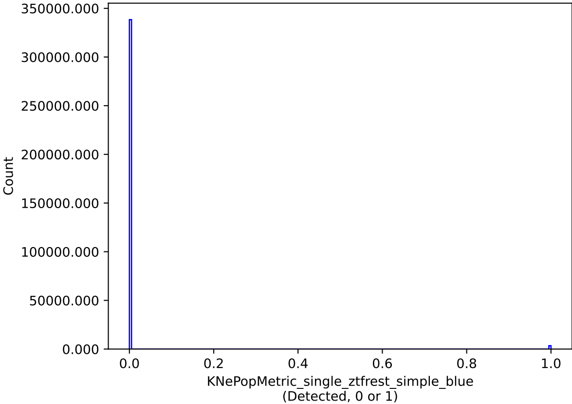
all_long_v3.4_10yrs single model: KNePopMetric_single_ztfrest_simple_blue
