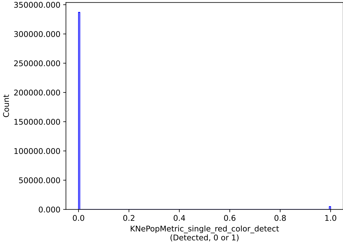
all_long_v3.4_10yrs single model: KNePopMetric_single_red_color_detect
