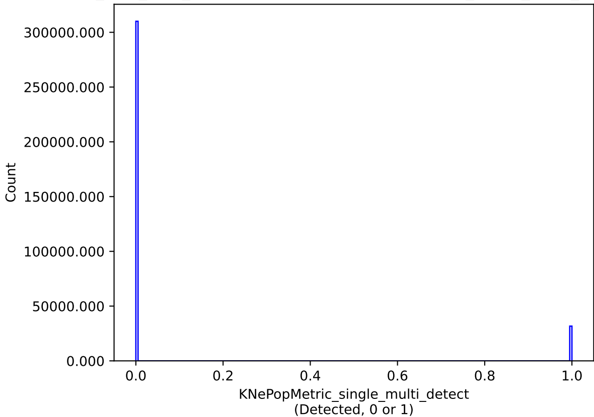
all_long_v3.4_10yrs single model: KNePopMetric_single_multi_detect
