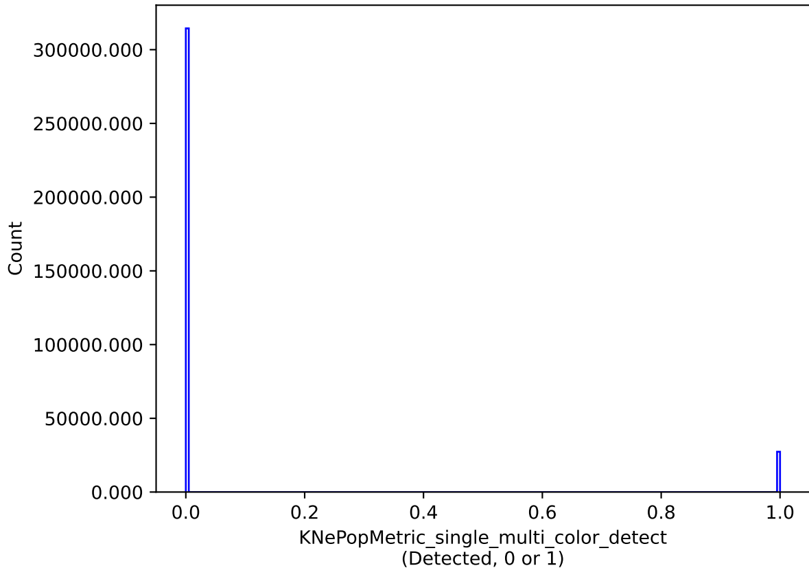
all_long_v3.4_10yrs single model: KNePopMetric_single_multi_color_detect
