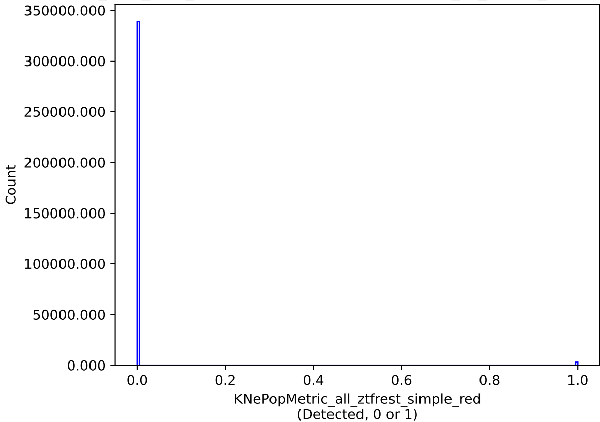
all_long_v3.4_10yrs all models: KNePopMetric_all_ztfrest_simple_red
