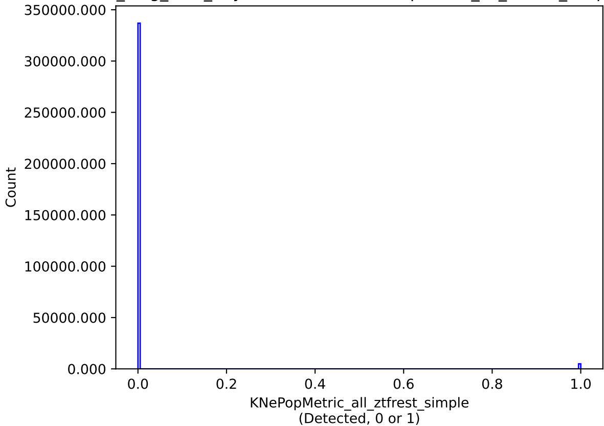
all_long_v3.4_10yrs all models: KNePopMetric_all_ztfrest_simple
