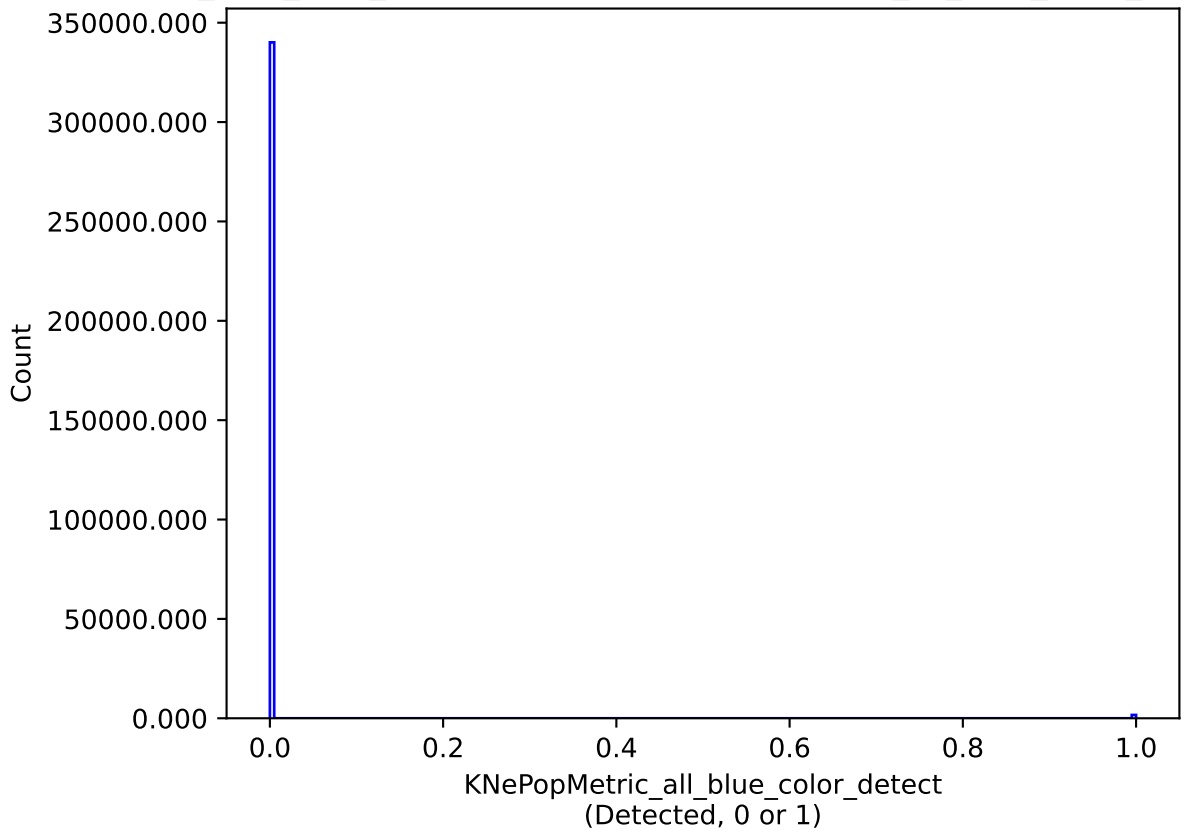
all_long_v3.4_10yrs all models: KNePopMetric_all_blue_color_detect
