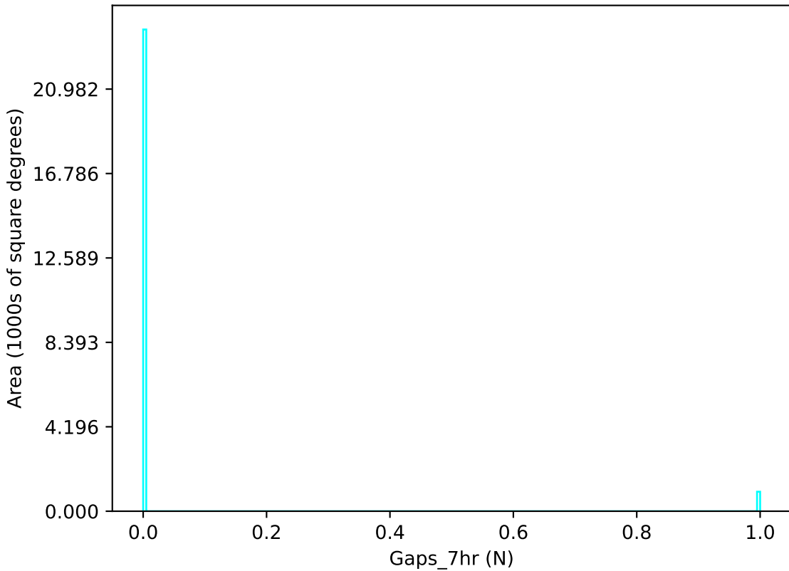
all_long_v3.4_10yrs u band: Gaps_7hr
