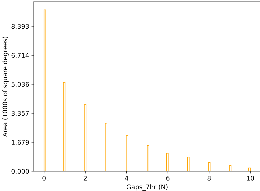
all_long_v3.4_10yrs r band: Gaps_7hr
