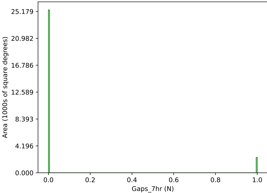
all_long_v3.4_10yrs g band: Gaps_7hr
