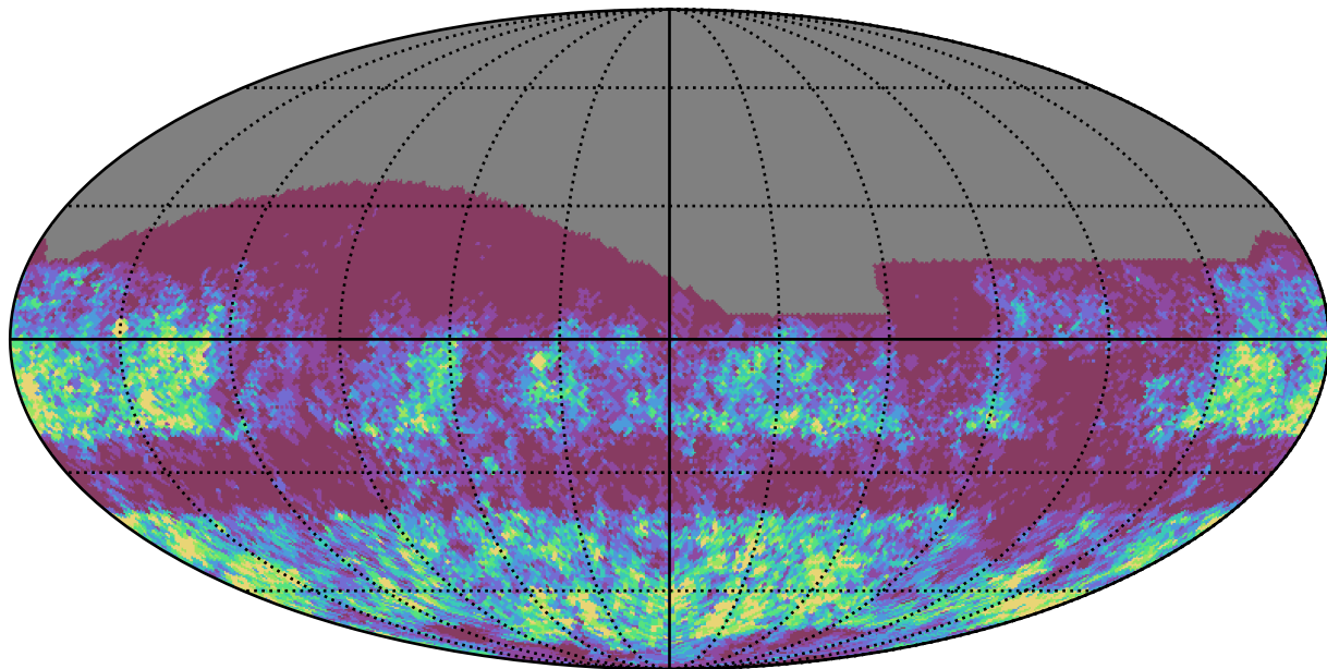
all_long_v3.4_10yrs z band: Gaps_3hr
