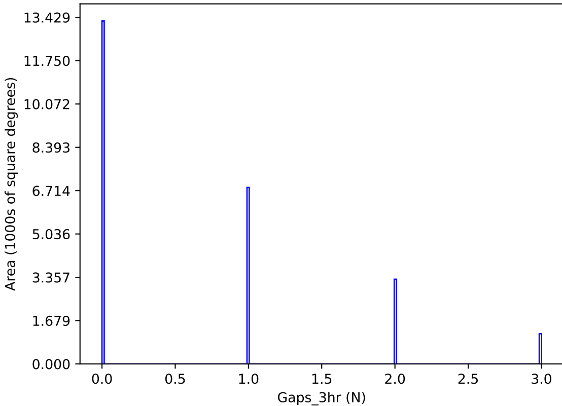
all_long_v3.4_10yrs y band: Gaps_3hr
