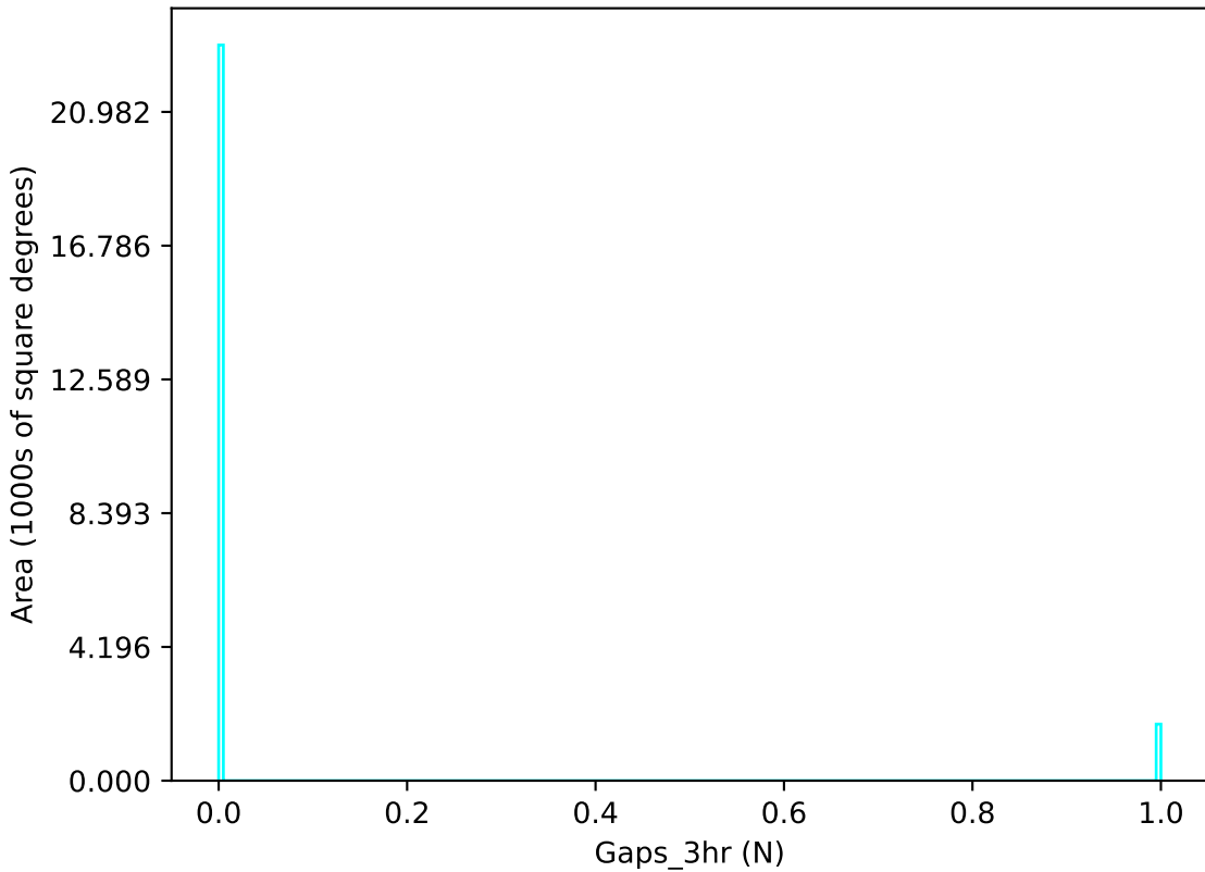
all_long_v3.4_10yrs u band: Gaps_3hr
