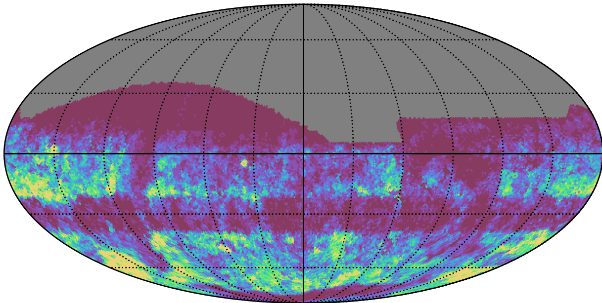
all_long_v3.4_10yrs r band: Gaps_3hr
