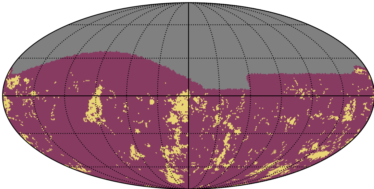
all_long_v3.4_10yrs g band: Gaps_3hr
