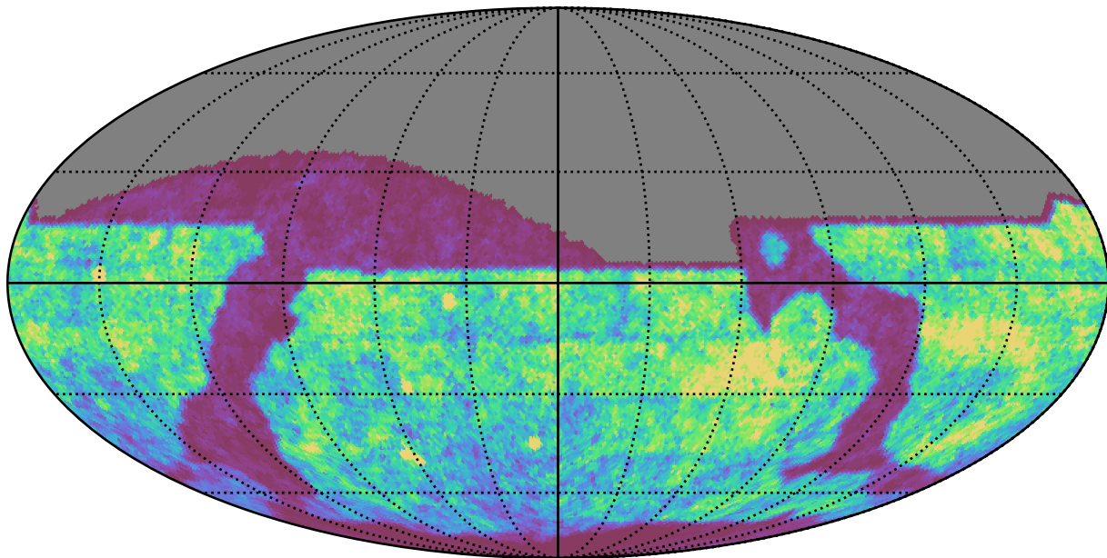
all_long_v3.4_10yrs r band: Gaps_24hr
