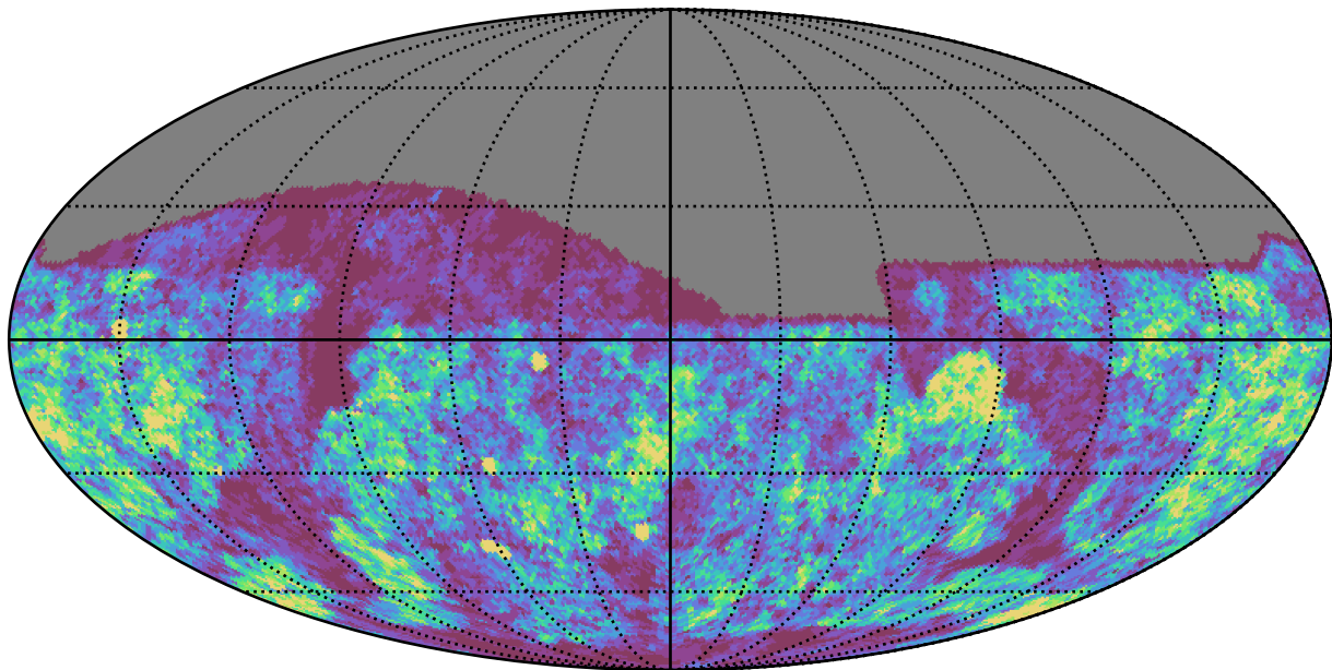
all_long_v3.4_10yrs g band: Gaps_24hr
