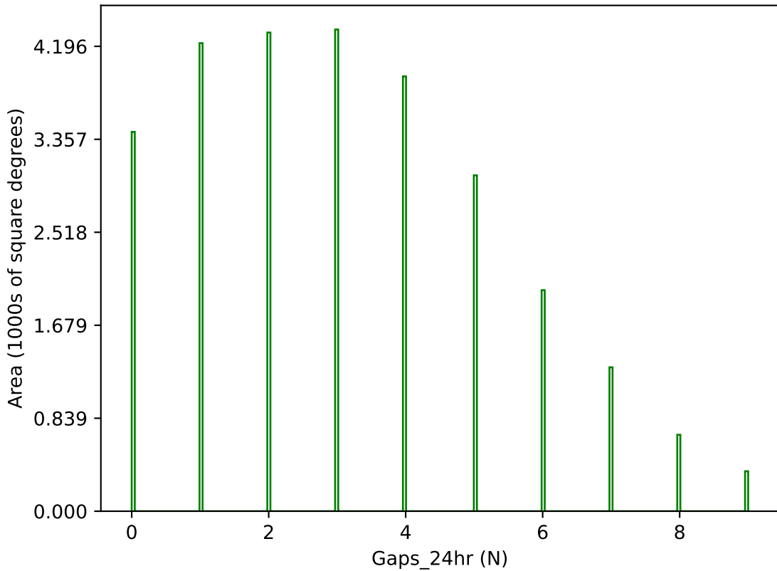
all_long_v3.4_10yrs g band: Gaps_24hr
