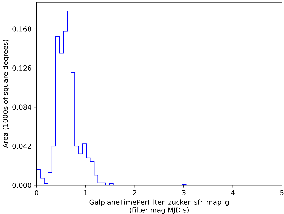
all_long_v3.4_10yrs : GalplaneTimePerFilter_zucker_sfr_map_g
