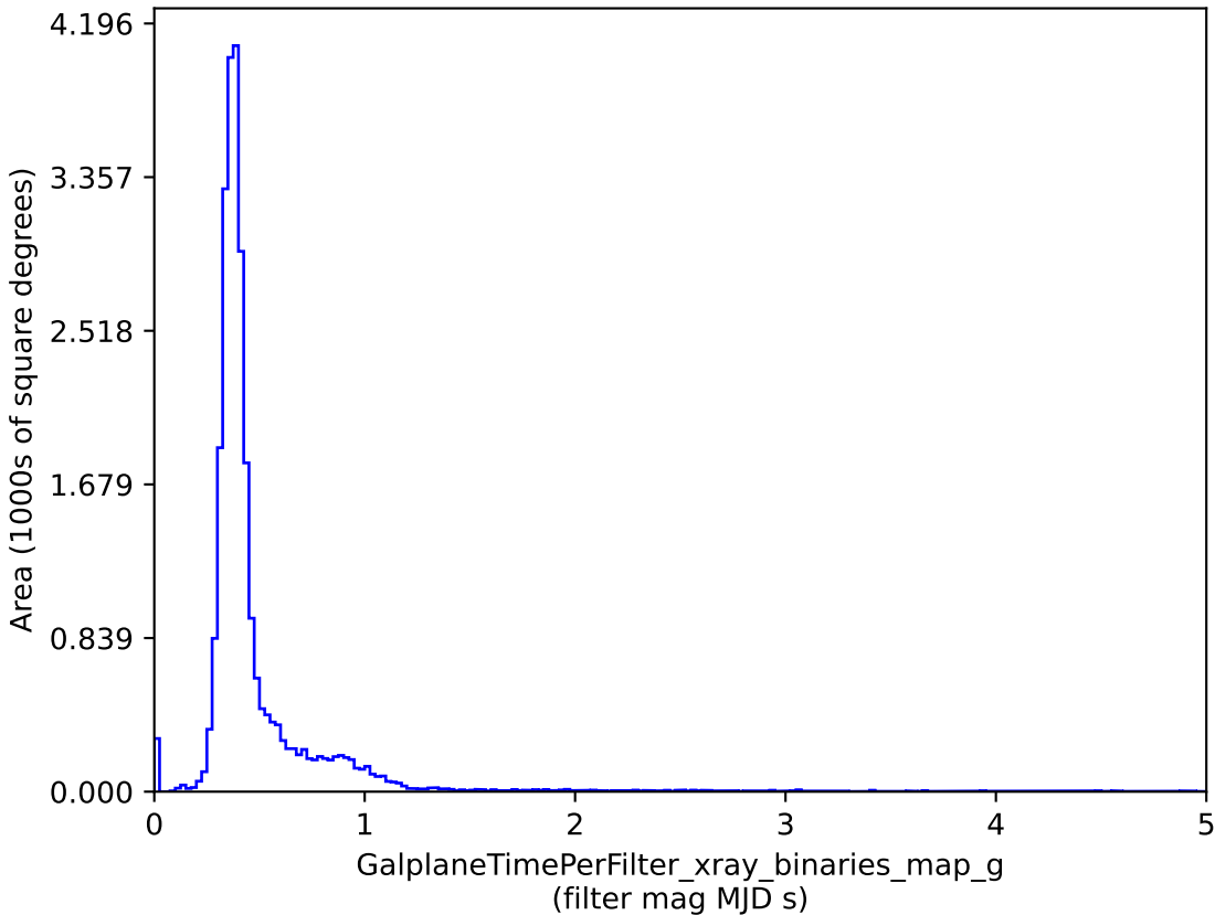
all_long_v3.4_10yrs : GalplaneTimePerFilter_xray_binaries_map_g
