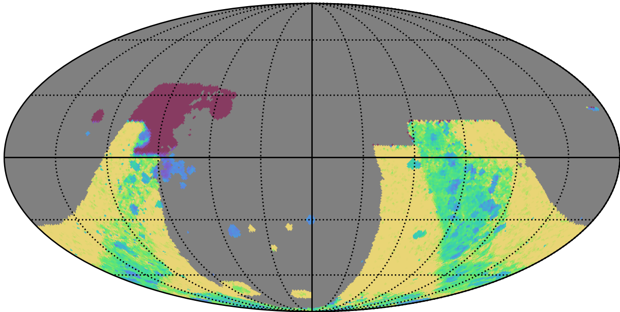
all_long_v3.4_10yrs : GalplaneTimePerFilter_combined_map_y
