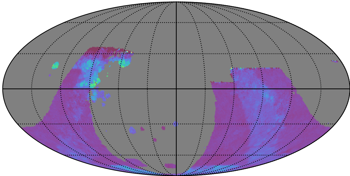
all_long_v3.4_10yrs : GalplaneTimePerFilter_combined_map_g
