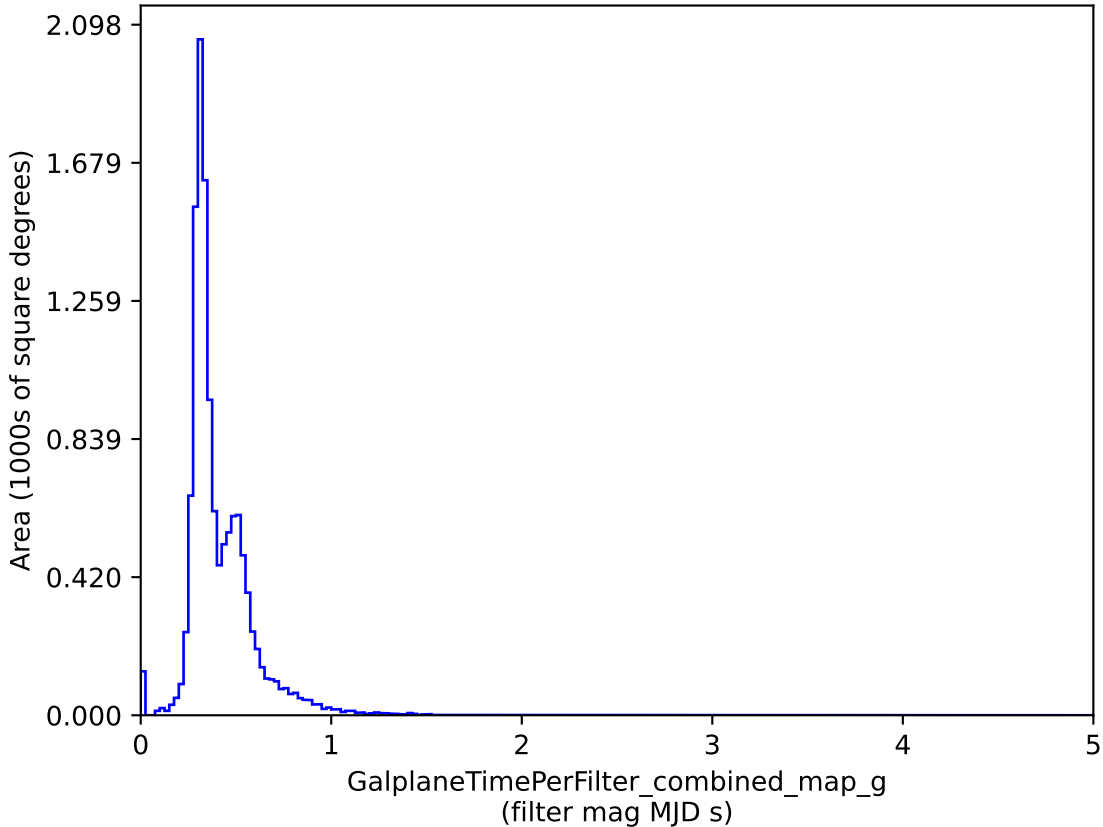
all_long_v3.4_10yrs : GalplaneTimePerFilter_combined_map_g
