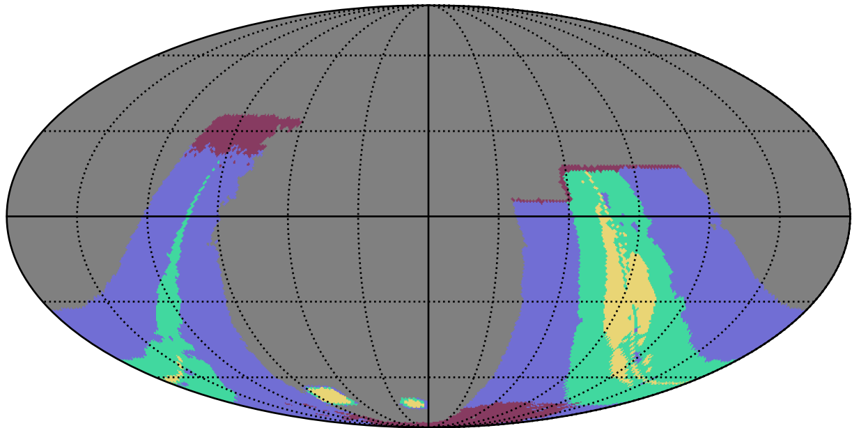
all_long_v3.4_10yrs : GalplaneFootprintMetric_galactic_plane_map_Tau_46_5
