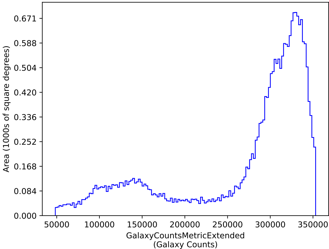
all_long_v3.4_10yrs y: GalaxyCountsMetricExtended
