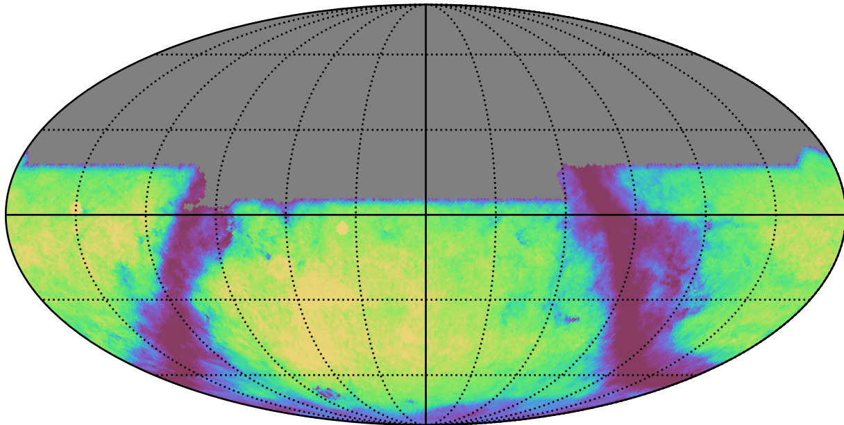
all_long_v3.4_10yrs u: GalaxyCountsMetricExtended
