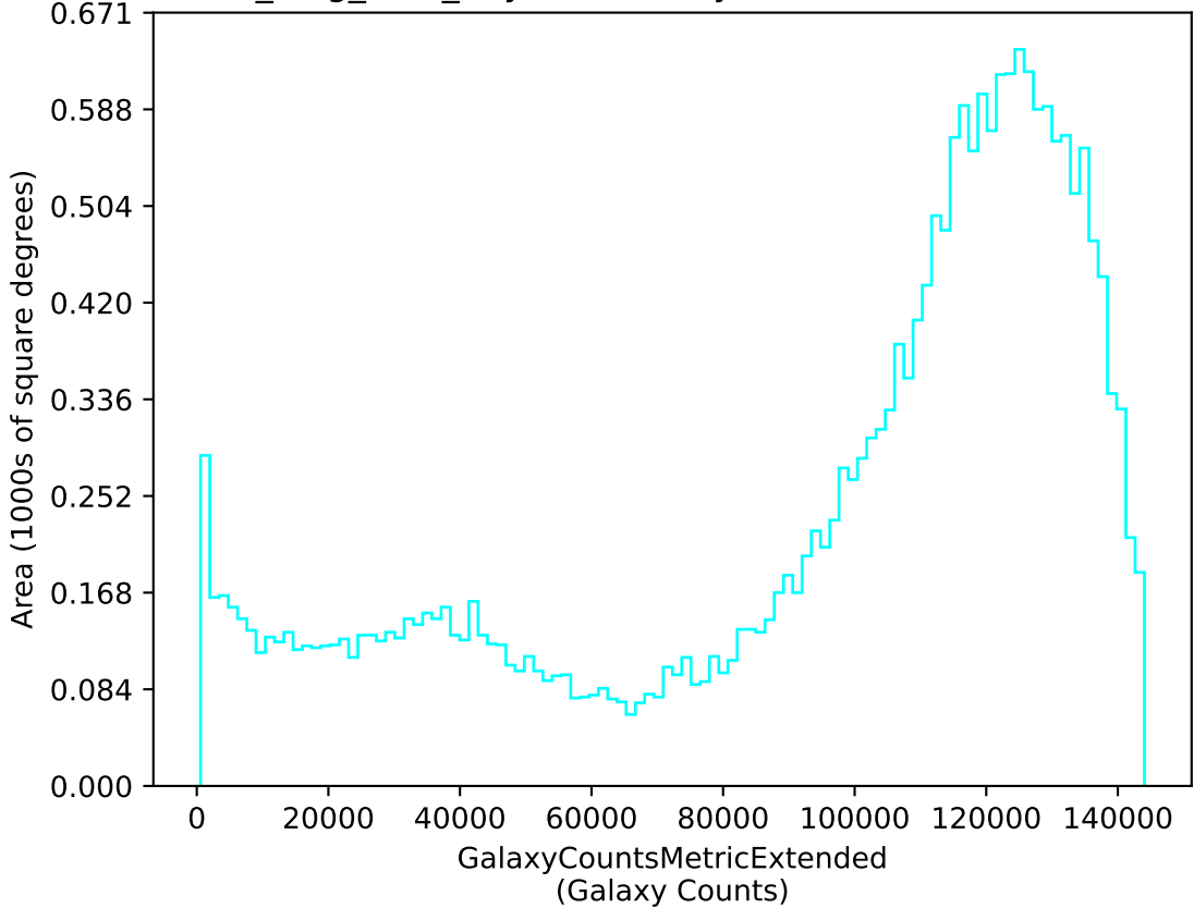
all_long_v3.4_10yrs u: GalaxyCountsMetricExtended
