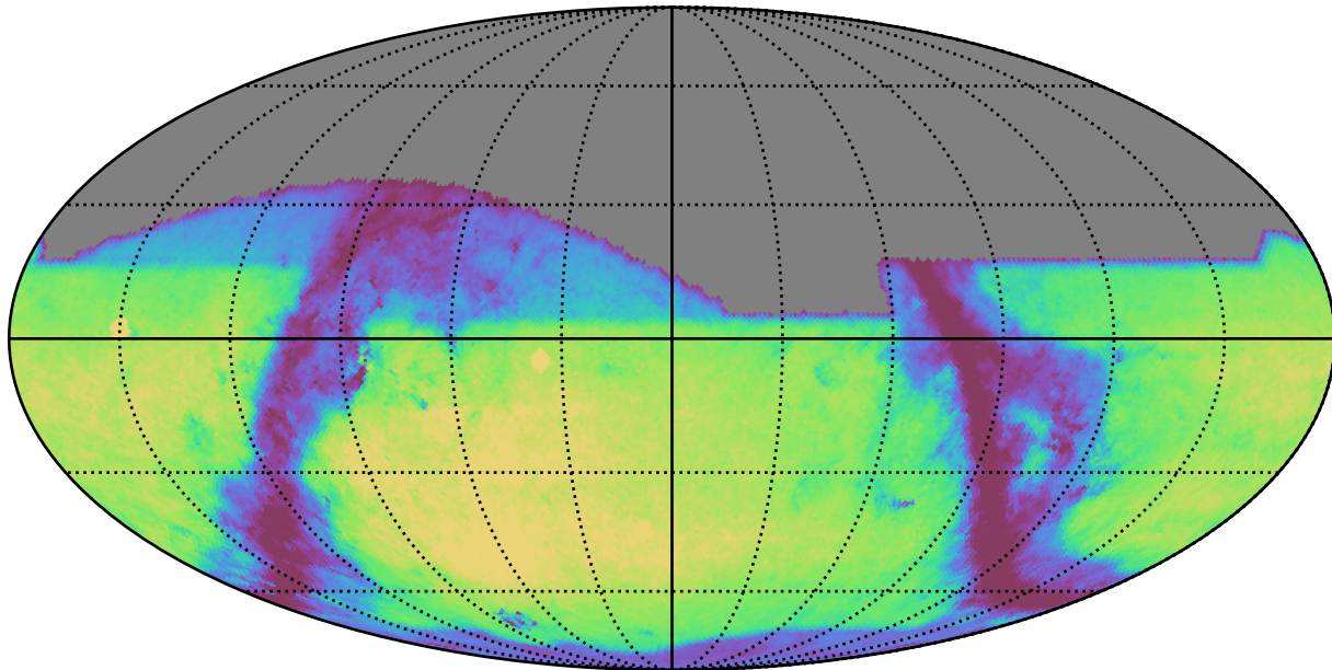
all_long_v3.4_10yrs r: GalaxyCountsMetricExtended
