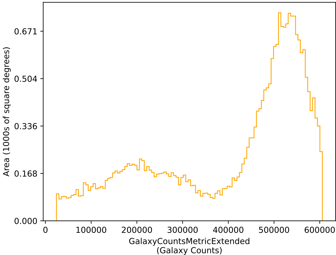
all_long_v3.4_10yrs r: GalaxyCountsMetricExtended
