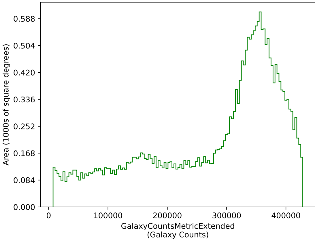
all_long_v3.4_10yrs g: GalaxyCountsMetricExtended
