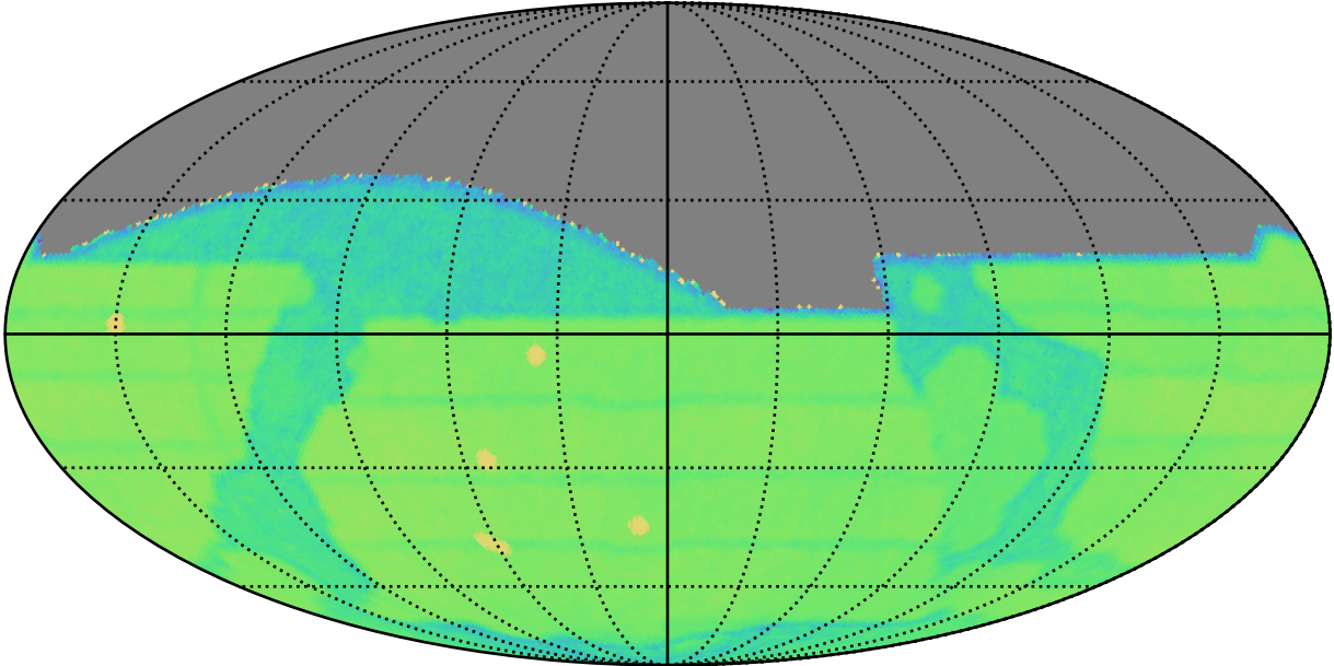
all_long_v3.4_10yrs : GalPlaneVisitIntervalsTimescales_xray_binaries_map_Tau_2_0
