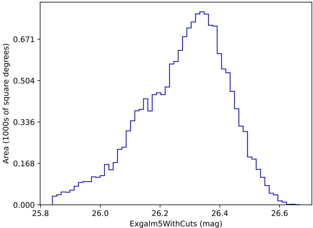
all_long_v3.4_10yrs i band non-DD year 9: ExgalM5WithCuts
