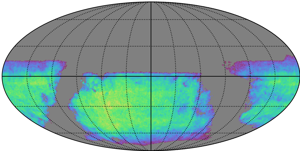
all_long_v3.4_10yrs i band non-DD year 8: ExgalM5WithCuts
