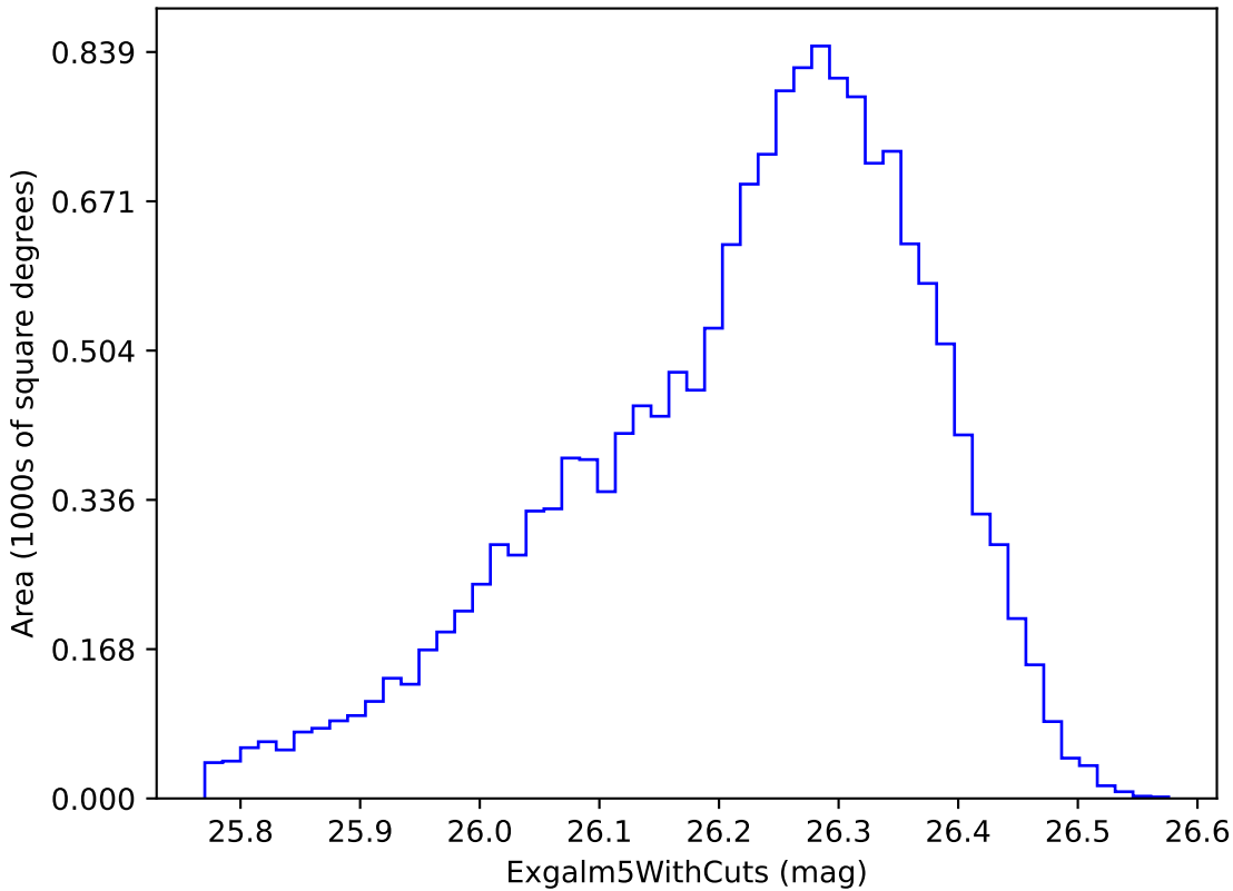
all_long_v3.4_10yrs i band non-DD year 8: ExgalM5WithCuts
