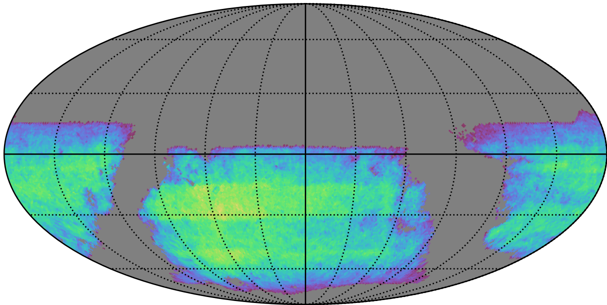
all_long_v3.4_10yrs i band non-DD year 7: ExgalM5WithCuts
