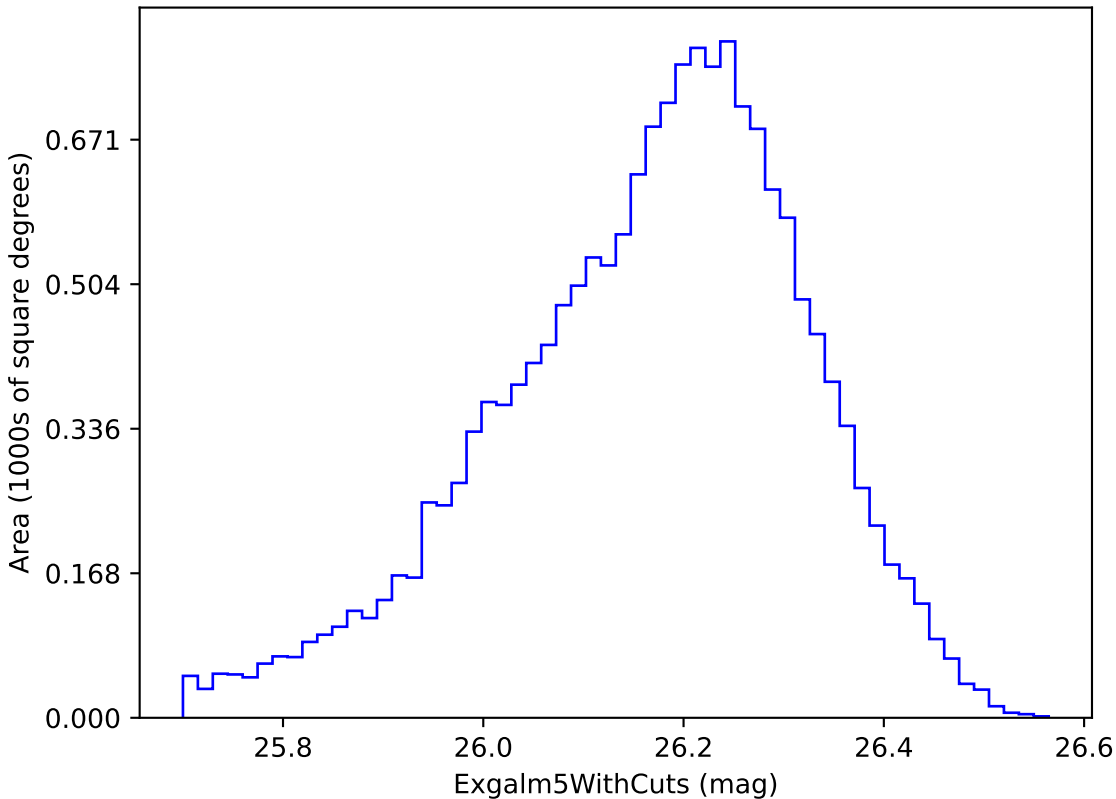
all_long_v3.4_10yrs i band non-DD year 7: ExgalM5WithCuts
