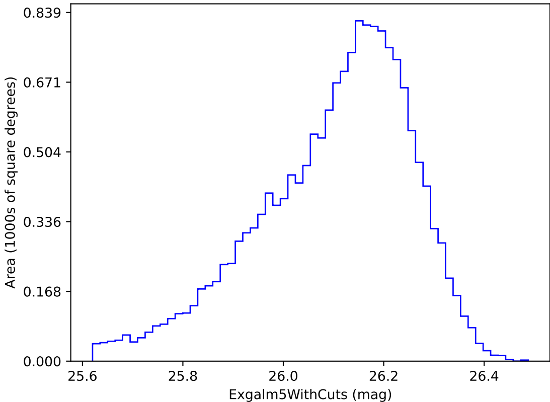
all_long_v3.4_10yrs i band non-DD year 6: ExgalM5WithCuts
