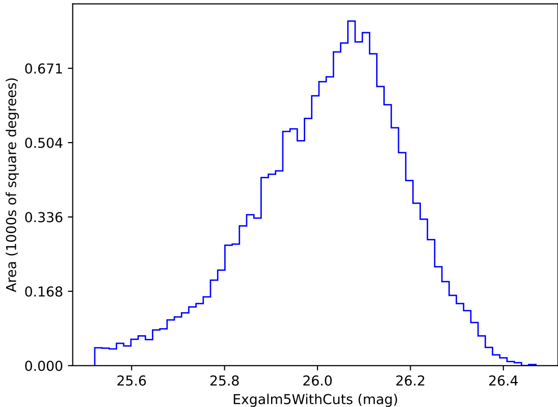
all_long_v3.4_10yrs i band non-DD year 5: ExgalM5WithCuts
