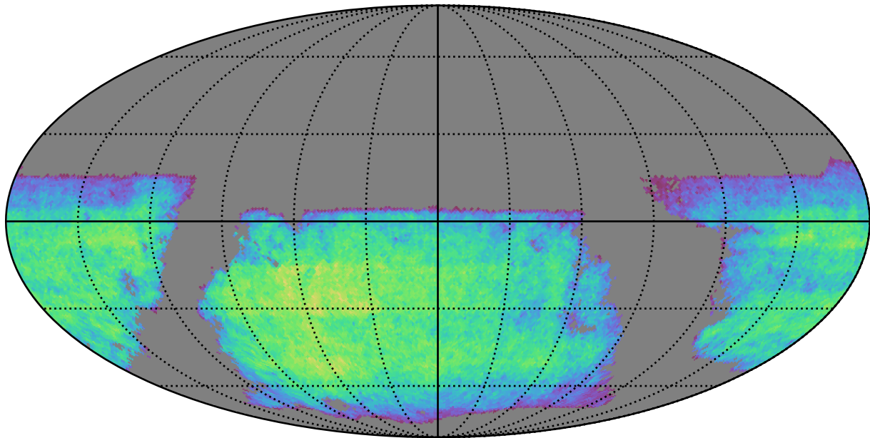
all_long_v3.4_10yrs i band non-DD year 4: ExgalM5WithCuts
