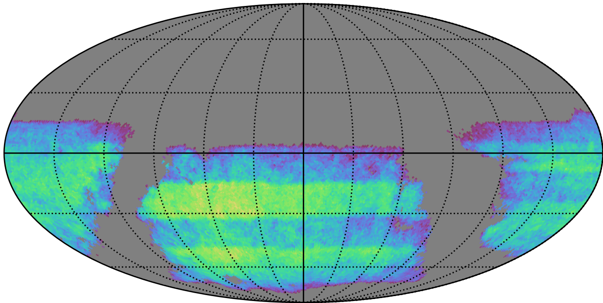
all_long_v3.4_10yrs i band non-DD year 3: ExgalM5WithCuts
