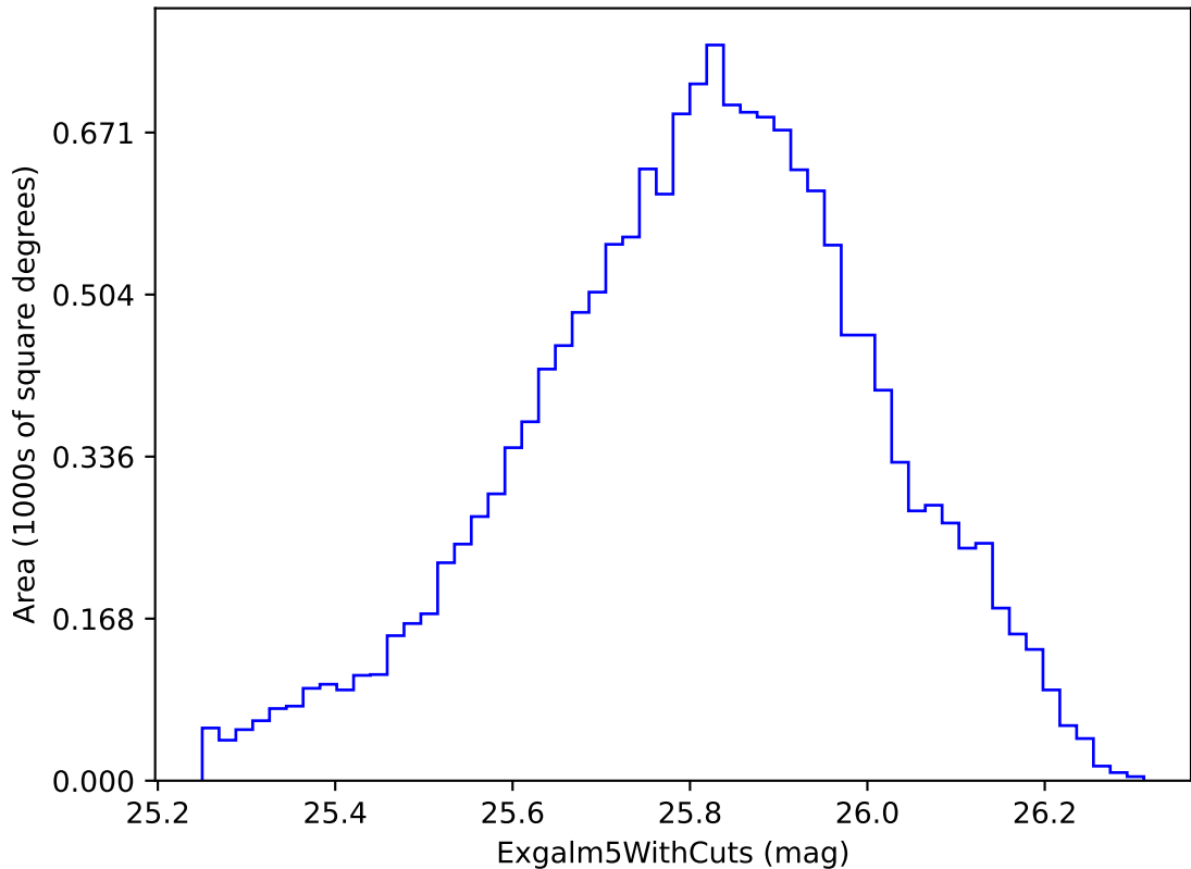
all_long_v3.4_10yrs i band non-DD year 3: ExgalM5WithCuts
