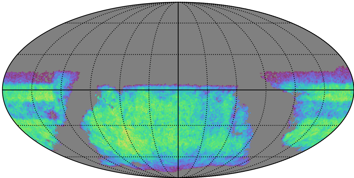
all_long_v3.4_10yrs i band non-DD year 2: ExgalM5WithCuts
