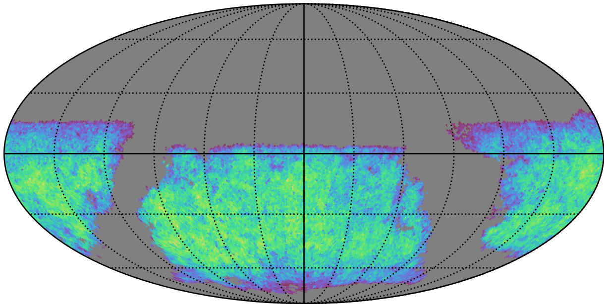
all_long_v3.4_10yrs i band non-DD year 1: ExgalM5WithCuts
