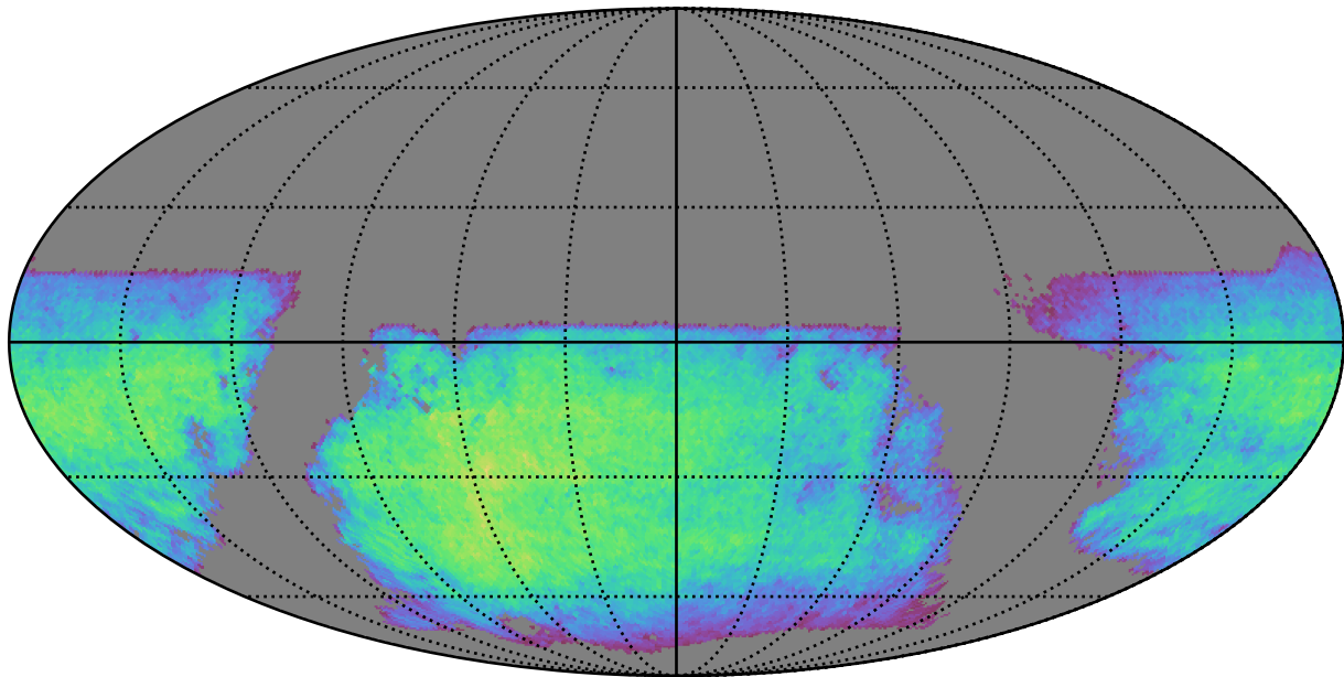
all_long_v3.4_10yrs i band non-DD year 10: ExgalM5WithCuts
