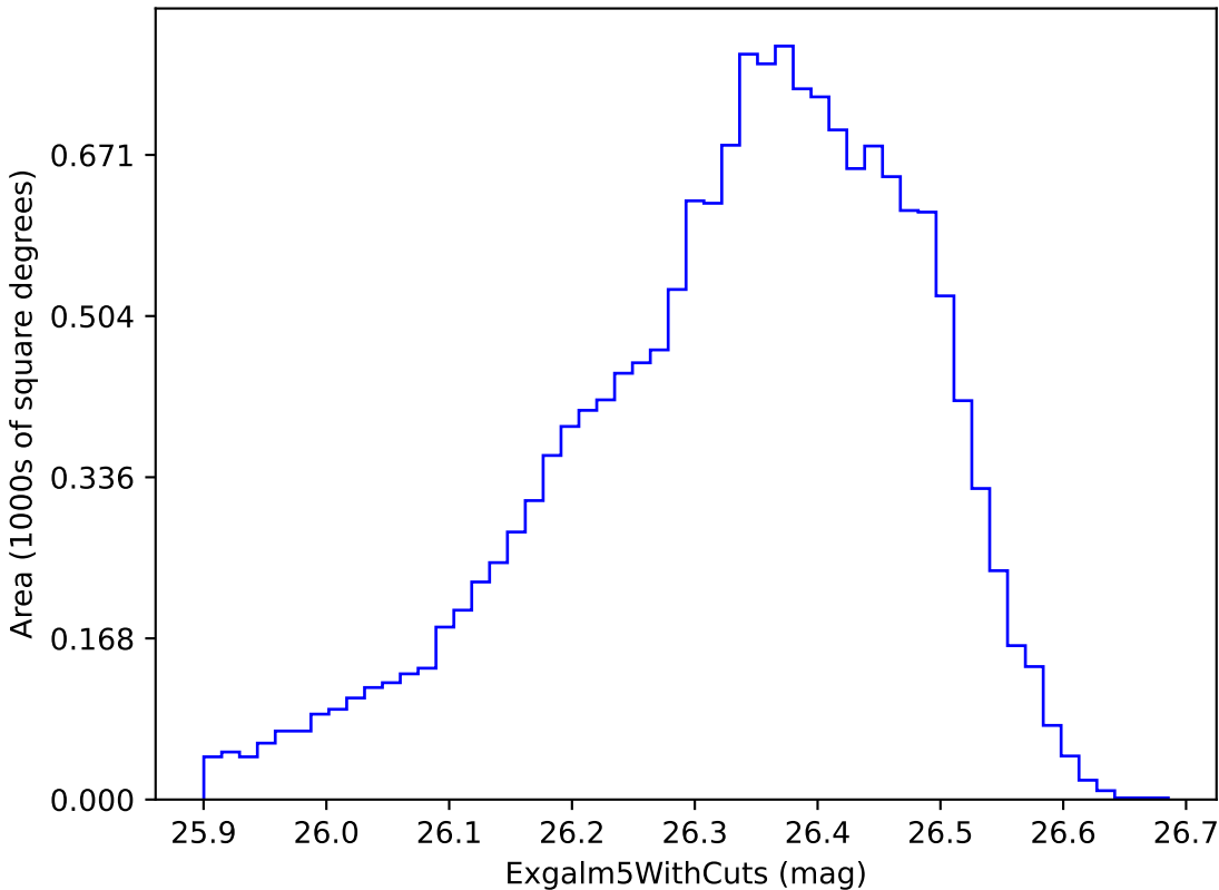
all_long_v3.4_10yrs i band non-DD year 10: ExgalM5WithCuts
