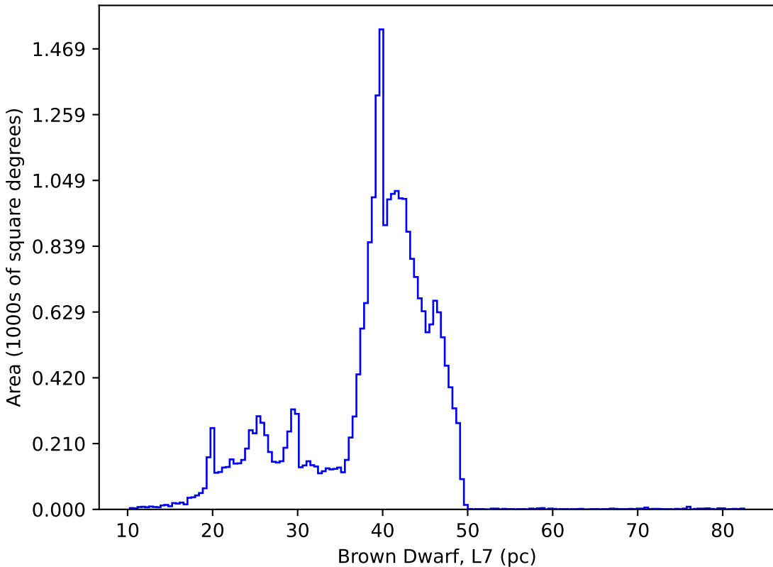
all_long_v3.4_10yrs : Brown Dwarf, L7
