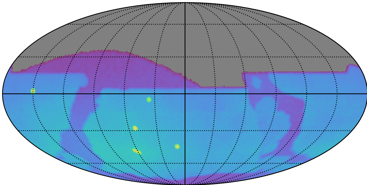
all_long_v3.4_10yrs : Brown Dwarf, L4
