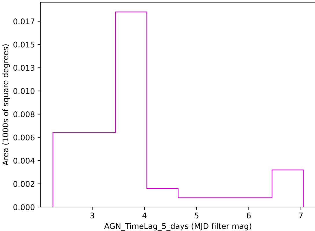
all_long_v3.4_10yrs z band: AGN_TimeLag_5_days
